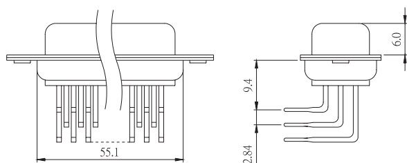
50 POSITION FEMALE
