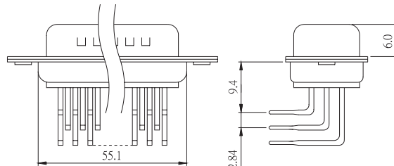
50 POSITION MALE
