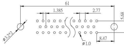
50 POSITION FEMALE/MALE
