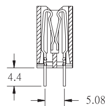
(CLOSE TYPE)
