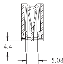
(OPEN TYPE)
